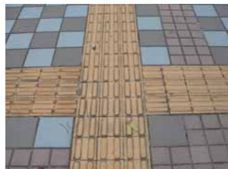
Fig. 27: Failure to Install Warning Blocks Where Directional Blocks Intersect (Taipei, Taiwan)
