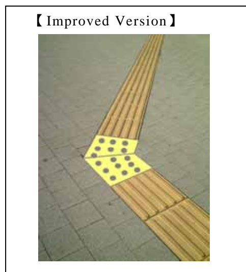
Fig. 41: The angle here is 130^\circ so warning blocks should be installed as in the improved version. ( Kanagawa, Japan )
